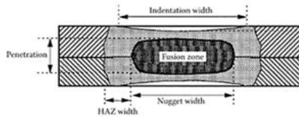
Figure.1 Weld attributes revealed by metallographic sectioning
