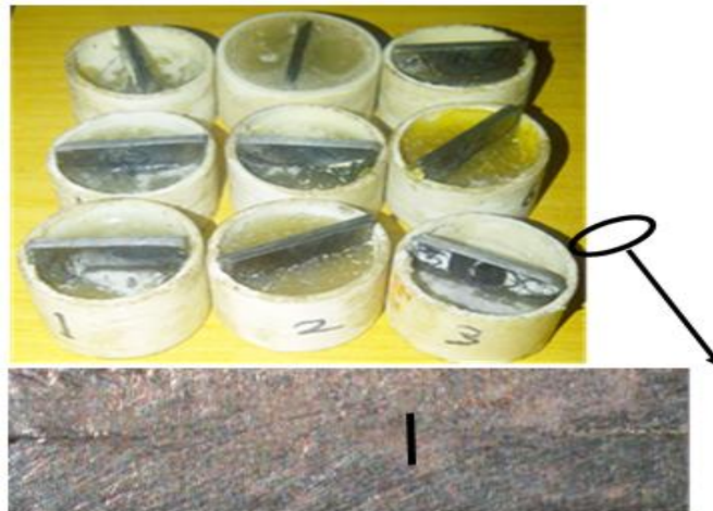
Figure.5 Arrangement for microscope view and one of microscopic image for measuring the nugget diameter
