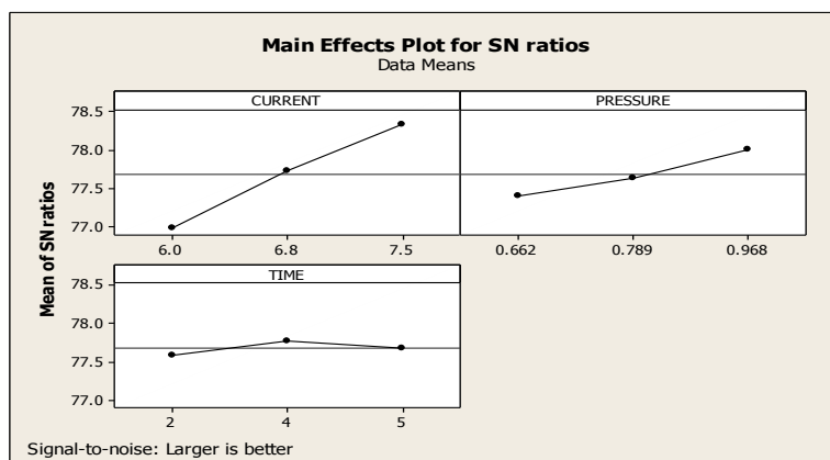
Figure.6 Main effects plot for s/n ratio.
