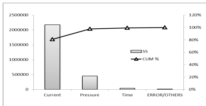
Figure.8 pareto chart of contributing factors
