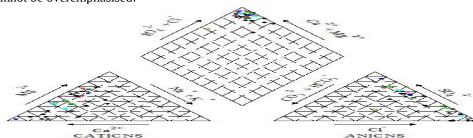
Figure 4: Piper diagram of groundwater from the study area
