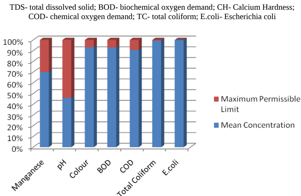
Figure 3: Correlation analysis between mean concentration and the recommended maximum permissible limits of (WHO, 2006; NSDWQ, 2007)
