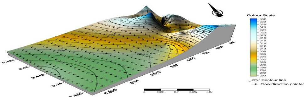
Fig.4: Groundwater flownet of the area
