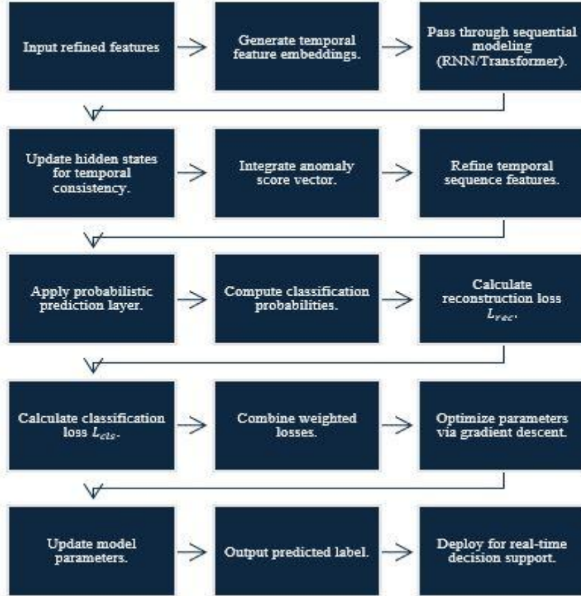
Fig.3. Temporal Modeling and Optimization Workflow for Real-Time Decision Support
