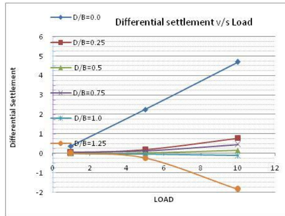
Figure. 4 Variation of Differential settlement with Load for e/B=0.2
